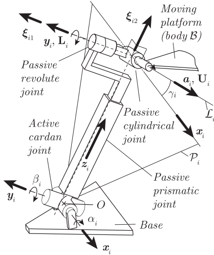
Fig. 3. A \underline{UPRC} kinematic chain.
