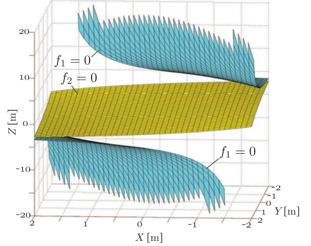
Fig. 7. Example of singularity loci when three perpendicular lines are observed (computed for a = 3.13, b = 3.13, c = -3.13 ).
