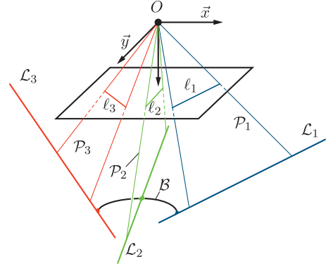
Fig. 2. Observation of three lines lying on a body B .
