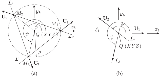
Fig. 5. Observation of three coplanar lines. (a) With no common intersection point. (b) With a common intersection point.
