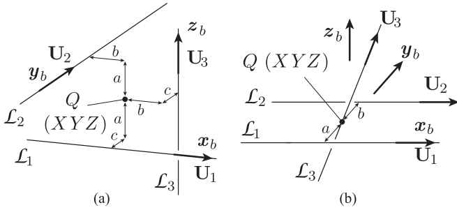
Fig. 6. Observation of lines in space. (a) No common intersection point. (b) Two lines are parallel.
