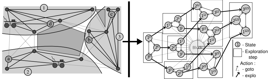
Figure 3. A partitioned Road-Map in 3 regions and the attached global MDP. For example, a state 2^{13} means that the robot is in the region 2 and the regions 1 and 3 are explored
