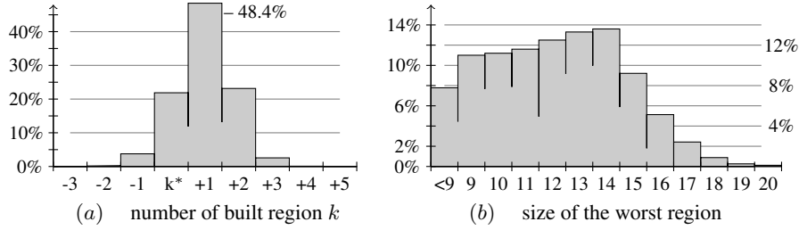
Figure 7. Classification of the experiments regarding the difference between the built k and the expected k^* number of regions and the size of the worst region in term of number of contained points of interest.
