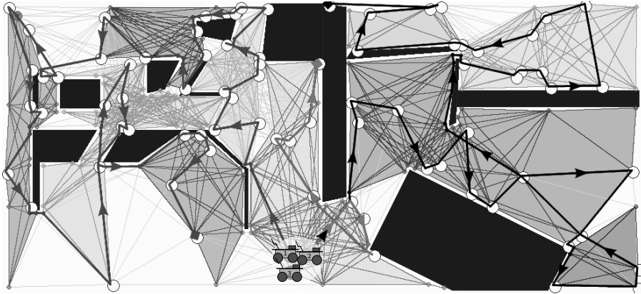
Figure 4. The 3 likely trajectories following the computed policy ( n_r = 3 , |I| = 80 and n_i^* = 10 ).
