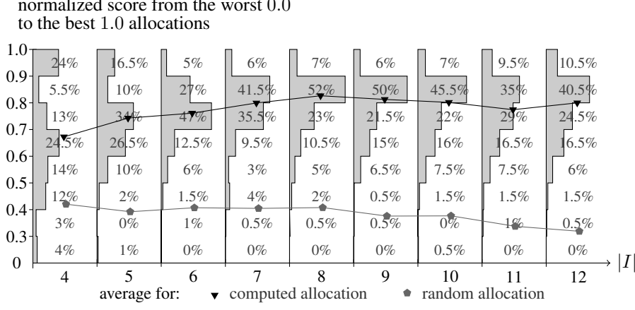
Figure 6. Population of obtained normalized scores by the allocation after partitioning. The population is presented for each considered number of points of interest |I|
