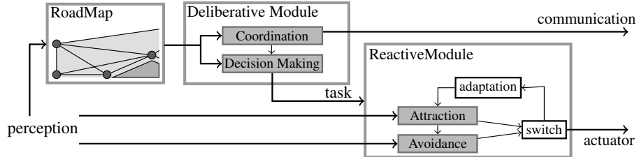
Figure 2. The Robot Architecture Schema.
