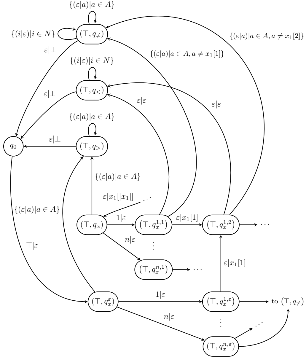
Figure 6. Structure of the (\top, x) -quarter of transducer \mathcal{A}_T : it accepts the relation \{(\top \cdot \sigma, u \cdot \perp) \mid u \in A^+ \setminus \{x(\sigma)\}\}^* .
