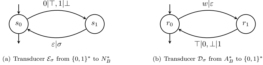
Figure 7. Encoder and decoders \mathcal{E}_{\sigma} and \mathcal{D}_{\sigma} , where \sigma is a solution of the instance \mathcal{I} of PCP and w the corresponding word.
