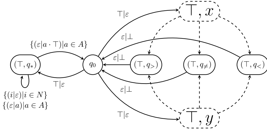
Figure 5. Structure of the \top -half of \mathcal{A}_T .
