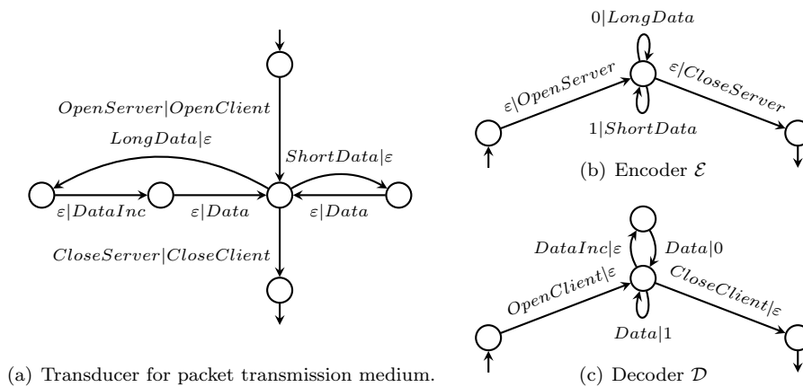
Figure 8. A channel of delay 0 for the packet transmission protocol.
