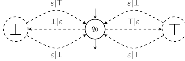
Figure 4. Symmetrical structure of \mathcal{A}_T .
