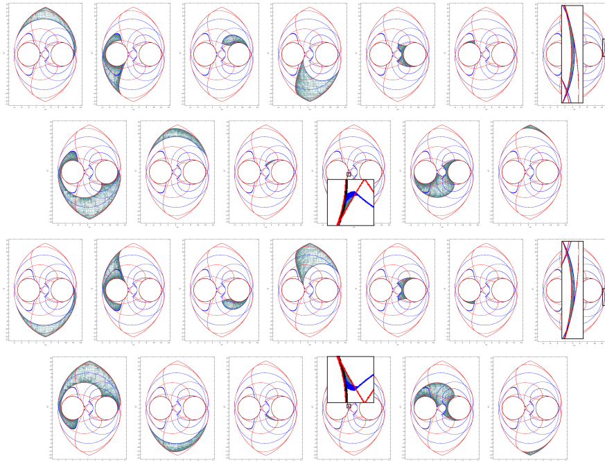
Figure 11: Computed CSNCs of \underline{RRRRR} with a circular obstacle.
