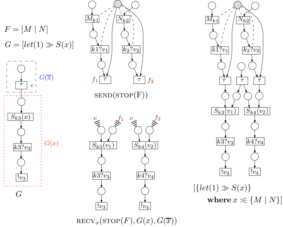
Fig. 2. Heap Construction Example: The shaded condition is the (\perp, \text{stop}) condition introduced by the STOP operator. A dashed arrowhead to a minimal condition of the RECV heap from an event name states that the condition depends on that external event. The external events here are e and f_1, f_2 in heaps G(\bar{x}) and \text{SEND}(\text{STOP}(F)) respectively. When these heaps are combined in the right most heap, these events become internal events.
