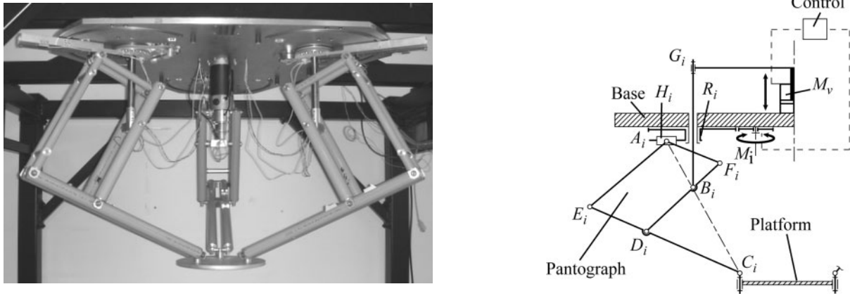
Fig. 10. The PAMINSA parallel robot: (a) prototype of the PAMINSA robot and (b) kinematic chain.
