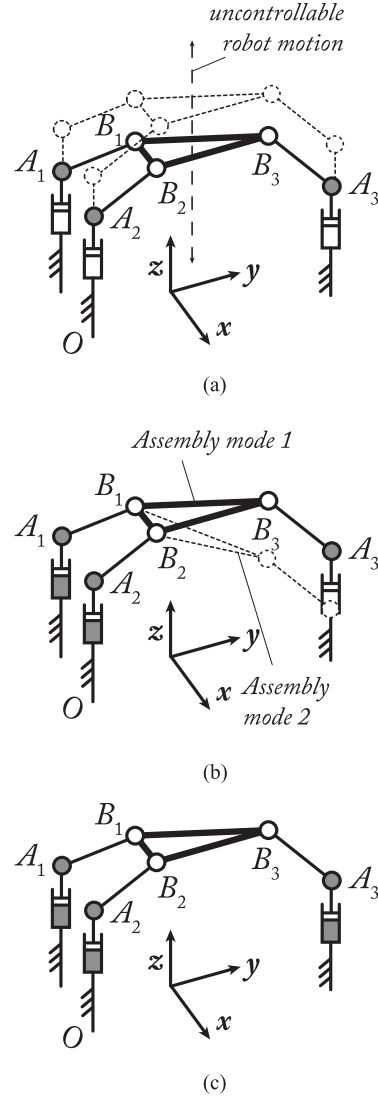
Fig. 21. Hidden robots involved in the tested visual servoings of the 3- PRS robot (projection in the yz plane – R and S joints at A_i and B_i , respectively, are drawn with the same symbol for the sake of clarity of the drawing). (a) When all leg directions \underline{u}_i are observed (Case 1): a 3- PRS robot. (b) When all leg directions \underline{u}_i and the Plücker coordinates of the line passing through the legs 1 and 2 are observed (Case 2): a {2- PRS }- PRS robot. (c) When all leg directions \underline{u}_i and the Plücker coordinates of the lines passing through the legs 1 and 3 are observed (Case 3): a 3- PRS robot.
