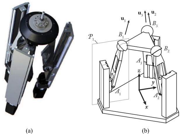
Fig. 20. Spatial 3- \underline{P} RS robot with parallel \underline{P} joints. (a) Design known as the Sprint Z3 machine. (b) Kinematic architecture.
