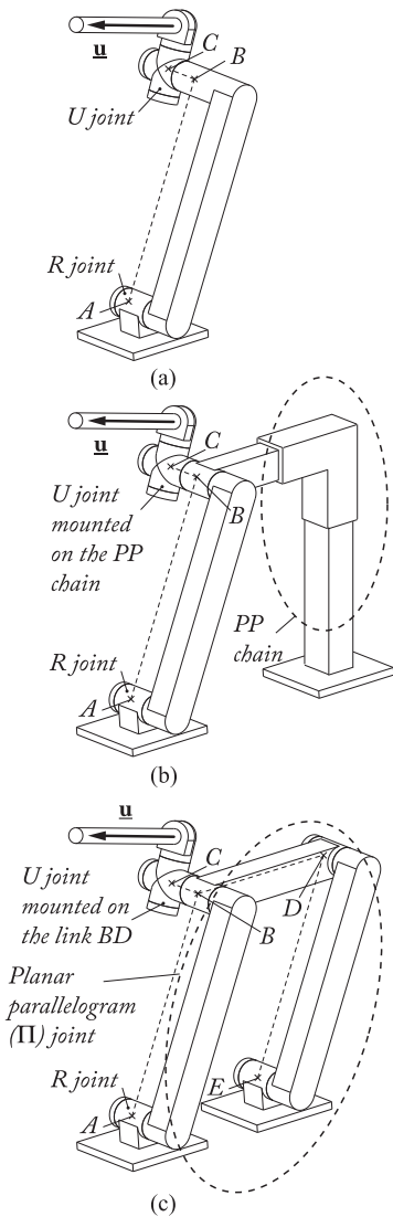
Fig. 5. RU leg and two equivalent solutions for its hidden leg. (a) A RU leg. (b) Virtual \{R-PP\}-U leg. (c) Virtual IIU leg.
