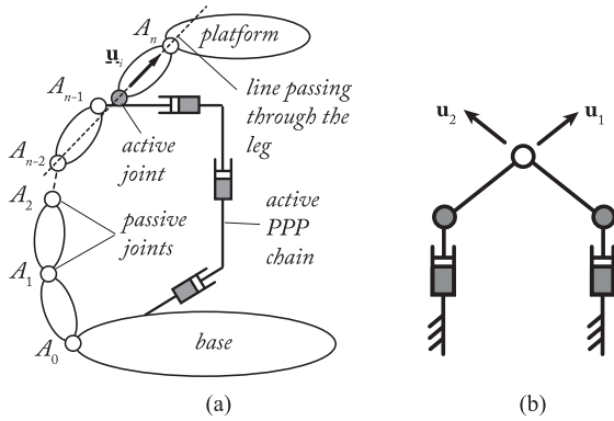
Fig. 16. Hidden robot leg when the Plücker coordinates of the line passing through the axis of the leg are observed. (a) For a general robot. (b) For the \underline{PRRRP} : a \underline{PRRRP} robot.
