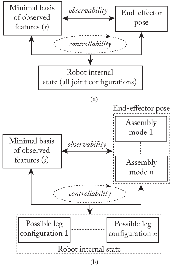
Fig. 2. Ensuring the observability and controllability of the robot through a proper feature observation. (a) When a global diffeomorphism exists. (b) When there is no global diffeomorphism.
