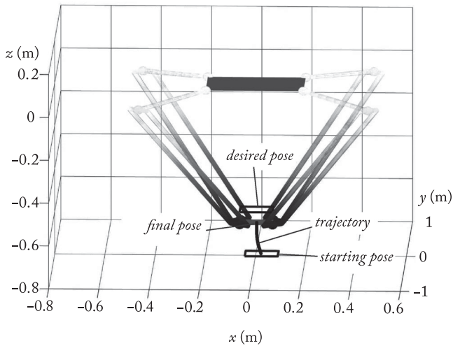
Fig. 14. Desired and final position of the Quattro when all legs are observed.
