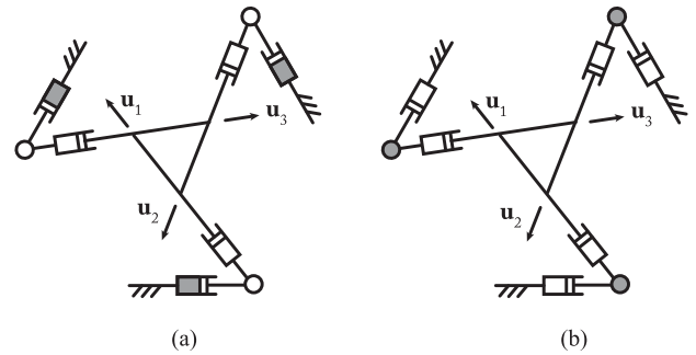
Fig. 11. 3-\underline{PRP} robot and its hidden robot model (the gray joints denote the actuated joints). (a) 3-\underline{PRP} robot. (b) Its hidden robot model: a 3-\underline{PRP} robot known to be uncontrollable.
