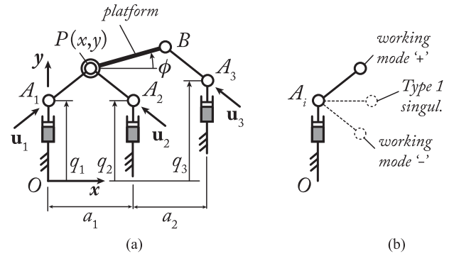
Fig. 17. Schematics of the 3- \underline{PRR} robot. (a) Kinematic architecture of the robot. (b) Kinematic architecture of one robot leg, its Type 1 singularity, and its working modes.
