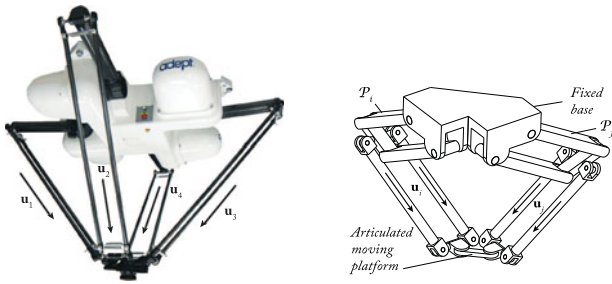
Fig. 13. Adept Quattro and its hidden robot model. (a) Adept Quattro: a 4-\underline{R}-2-U robot. (b) Its hidden robot model: a 2-\underline{II}-2-\underline{UU} robot (when two legs are observed).
