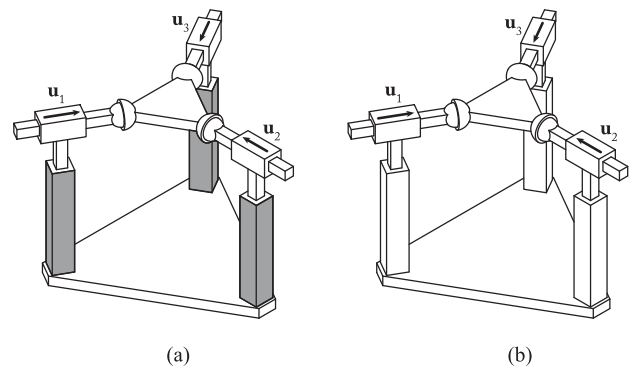
Fig. 8. 3- PPS robot and its hidden robot model (the gray joints denote the actuated joints). (a) 3- PPS robot. (b) Its hidden robot model: a 3- PPS robot with no actuators.
