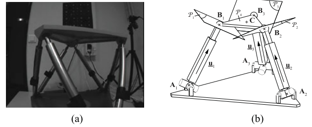
Fig. 12. G-S platform and its hidden robot model. (a) G-S platform from DeltaLab: a 6-\underline{UPS} robot. (b) Its hidden robot model: a 3-\underline{UPS} robot (when three legs are observed).
