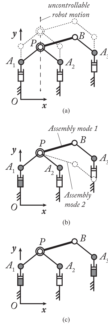
Fig. 19. Hidden robots involved in the tested visual servings of the 3- \underline{P}RR robot. (a) When all leg directions \underline{u}_i are observed (Case 1): a 3- \underline{P}RR robot. (b) When all leg directions \underline{u}_i and the Plücker coordinates of the line passing through the leg 1 are observed (Case 2): a \underline{P}RR -{2- \underline{P}RR } robot. (c) When all leg directions \underline{u}_i and the Plücker coordinates of the lines passing through the legs 1 and 3 are observed (Case 3): a \underline{P}RR -{2- \underline{P}RR } robot.
