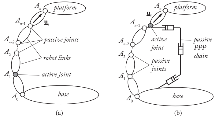
Fig. 3. (a) General robot leg and (b) its corresponding hidden robot leg when the vector \underline{u}_i is observed.
