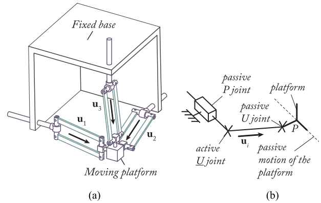
Fig. 15. Orthoglide and its hidden robot leg. (a) Kinematic chain. (b) The hidden robot leg.
