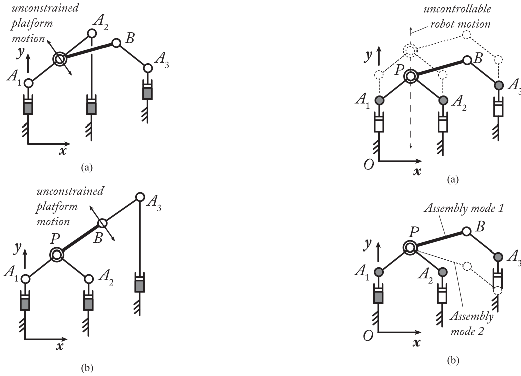
Fig. 18. Singularities of the 3- \underline{P}RR robot. (a) Example of the first case of Type 2 singularity. (b) Example of the second case of Type 2 singularity.
