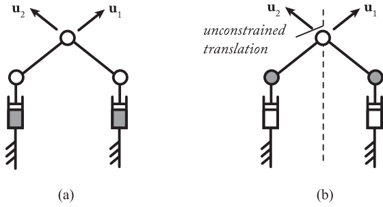
Fig. 9. \underline{PRRRP} robot and its hidden robot model (the gray circles denote the actuated joints). (a) \underline{PRRRP} robot. (b) Its hidden robot model: a \underline{PRRRP} robot.
