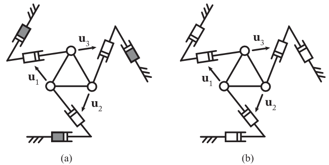
Fig. 7. 3- PPR robot and its hidden robot model (the gray joints denote the actuated joints). (a) 3- PPR robot. (b) Its hidden robot model: a 3- PPR robot with no actuators.
