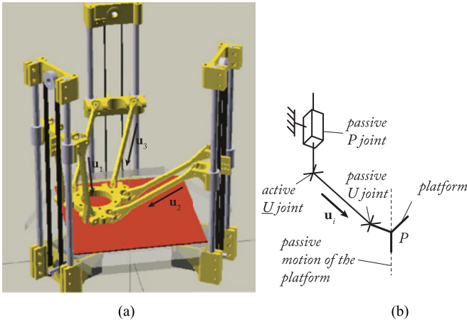
Fig. 10. UraneSX robot and its hidden robot leg. (a) Schematics of the architecture: a 3-\underline{PUU} robot with the three actuated P joints in parallel. (b) Its hidden robot leg: a \underline{PUU} leg; thus, the hidden robot is a 3-\underline{PUU} robot with the three passive P joints in parallel leading to an uncontrollable translation along the P joints direction.
