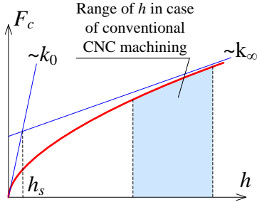
Figure 2 Fractional cutting force model F_c(h)
