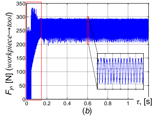
Figure 11 Variation of machining force components F_x (a) and F_y (b) for whole milling process
