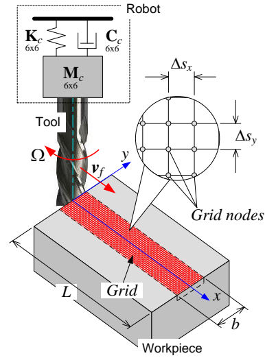
Figure 4 Meshing of the workpiece area
