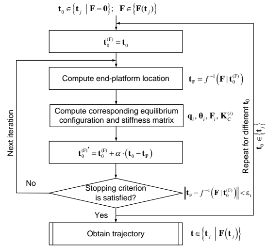
Figure 7 Procedure for compensation of compliance errors
