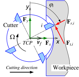
Figure 3 Forces of tool/workpiece interaction
