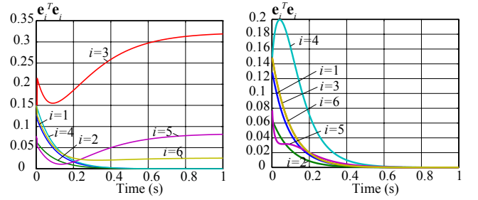
(a) when legs 1,2,4 are observed (b) when legs 2,3,6 are observed
